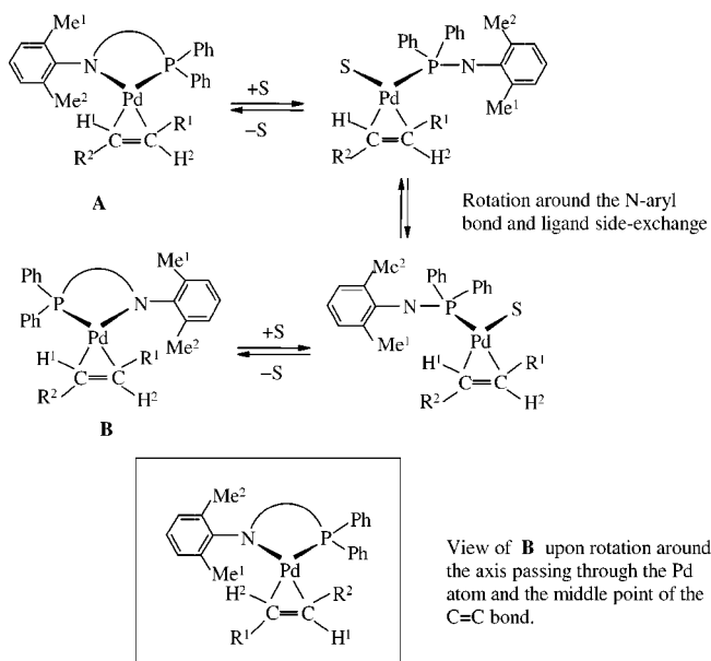
Scheme 4. Proposed mechanism for the dynamic behaviour of complex 3a ( \text{R}^1 = \text{R}^2 = \text{CO}_2\text{Me} ; S = solvent)
