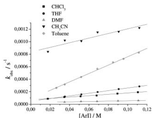
Figure 1. Plots of k_{\text{obs}} versus the aryl iodide concentration for the oxidative addition of ArI to complex 1a in different solvents at 25 °C in the presence of dmfu ( [\text{1a}]_0 = 1 \cdot 10^{-4} M; [\text{dmfu}] = 3 \cdot 10^{-3} M)
