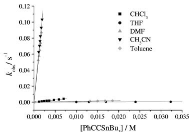
Figure 2. Plots of k_{\text{obs}} versus the stannane concentration for the transmetallation of 1c with \text{PhC}\equiv\text{CSnBu}_3 in different solvents at 25 °C in the presence of fn ( [\text{1c}]_0 = 1 \cdot 10^{-4} M; [\text{fn}] = 2 \cdot 10^{-4} M)
